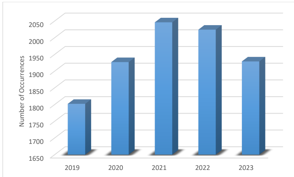
FIGURE 3: 2019 - 2023 Reported Assaults
